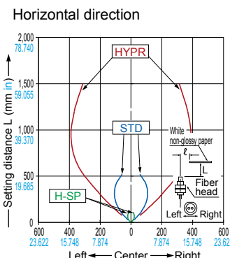
FD-62 Reflective type
