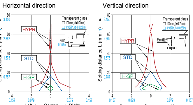
FD-H18-L31 Reflective type
