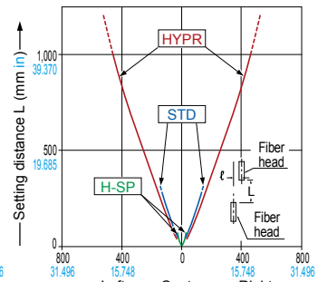
FT-H30-M1V-S Thru-beam type
