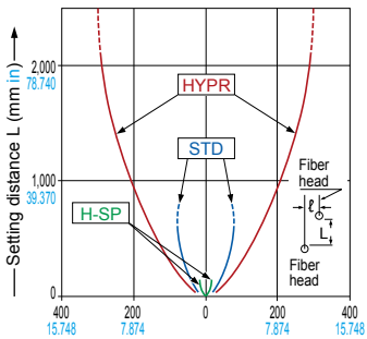
FT-H20-VJ50-S FT-H20-VJ80-S Thru-beam type
