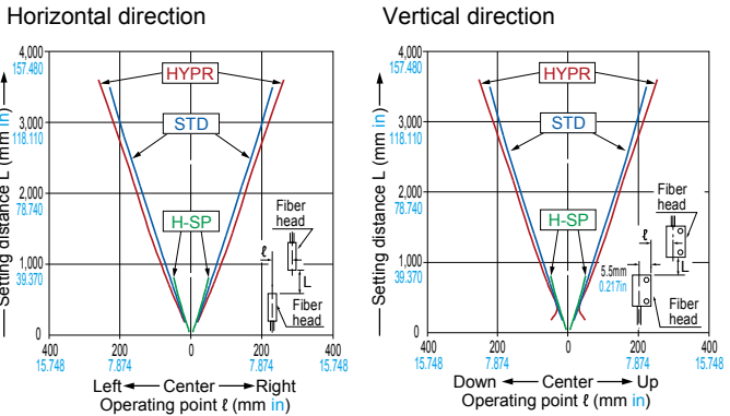
FT-Z30W Thru-beam type
