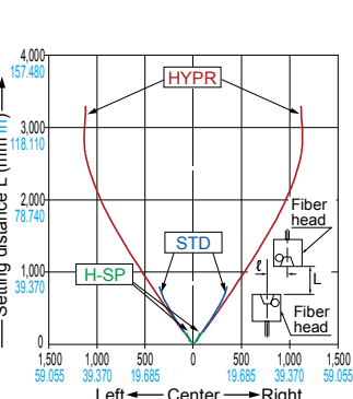
FT-Z40HBW Thru-beam type
