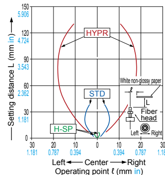
FD-R60 Reflective type
