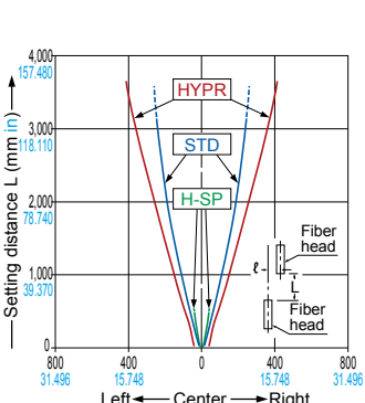
FT-Z802Y Thru-beam type
