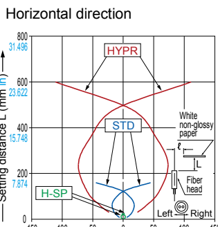
FD-S30 Reflective type
