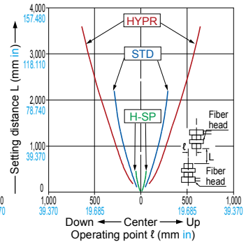
FT-S11
