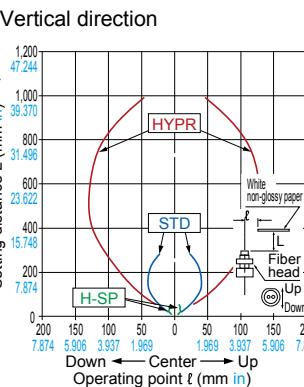
FD-S30 Reflective type
