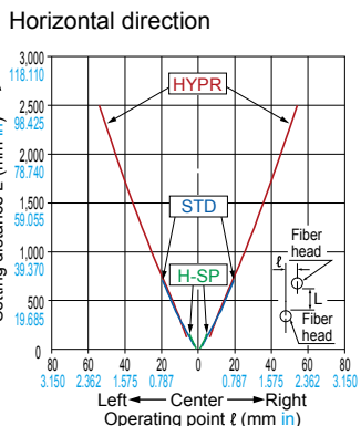
FT-KV40 Thru-beam type
