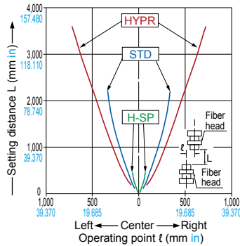
FT-R60Y
