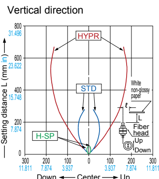
FD-64X Reflective type
