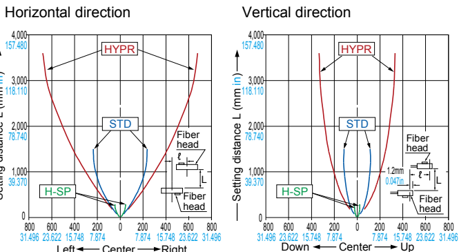
FT-Z40W Thru-beam type
