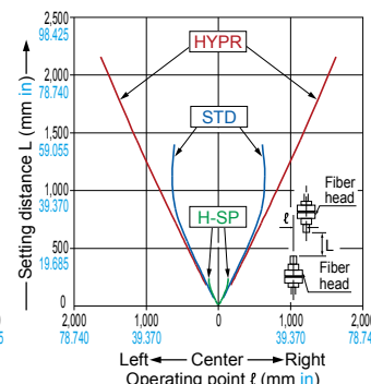
FT-A11H Thru-beam type
