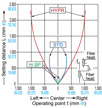
FT-H13-FM2 Thru-beam type
