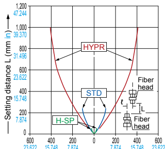
FT-R31 Thru-beam type
