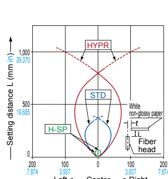
FD-H20-M1 Reflective type
