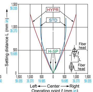
FT-A11V Thru-beam type
