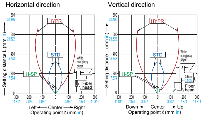
FD-E23 Reflective type
