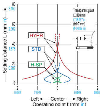
FD-H35-20S
