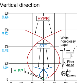
FD-S30 Reflective type
