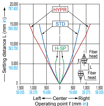
FT-31W Thru-beam type
