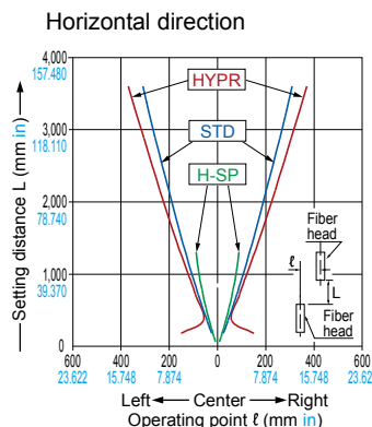
FT-A11H Thru-beam type
