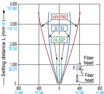
FT-L80Y Thru-beam type
