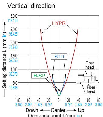
FT-KV40 Thru-beam type
