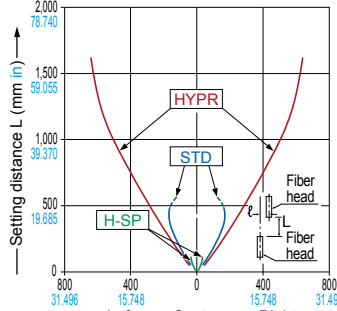
FT-H20W-M1 Thru-beam type
