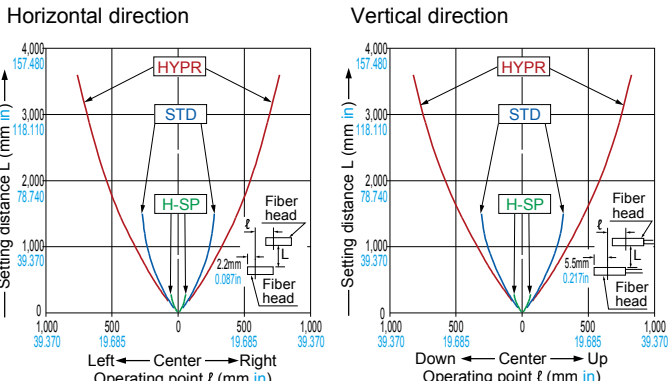
FT-Z40HBW Thru-beam type
