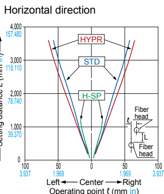
FT-L80Y Thru-beam type
