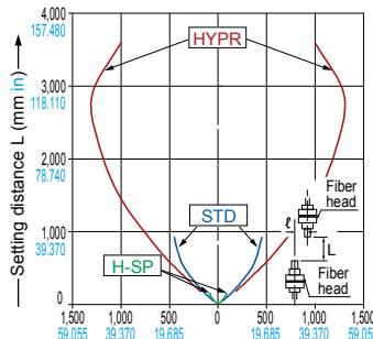
FT-R40 Thru-beam type
