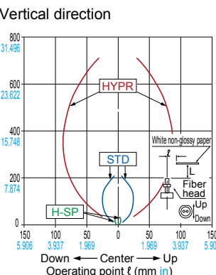
FD-R61Y Reflective type
