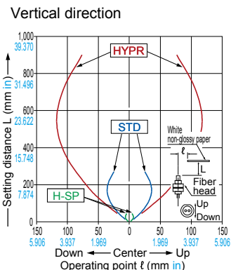
FD-64X Reflective type
