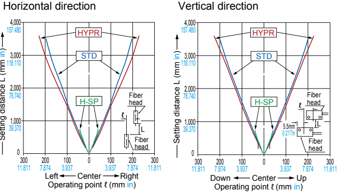
FT-Z30H Thru-beam type
