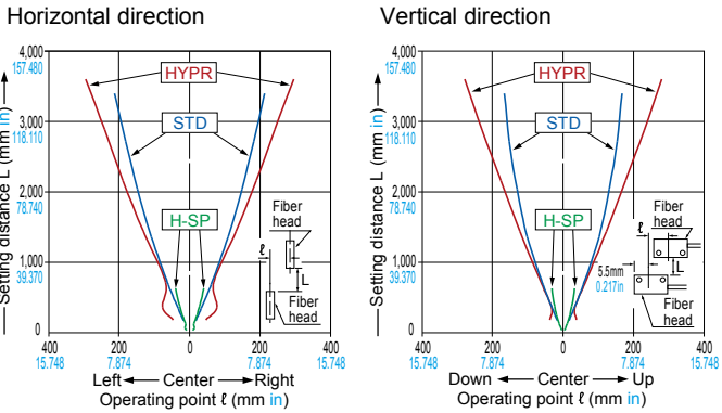
FT-Z30HW Thru-beam type
